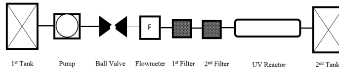
Figure 2: Diagram Process of Prototype Ballast Water Treatment
