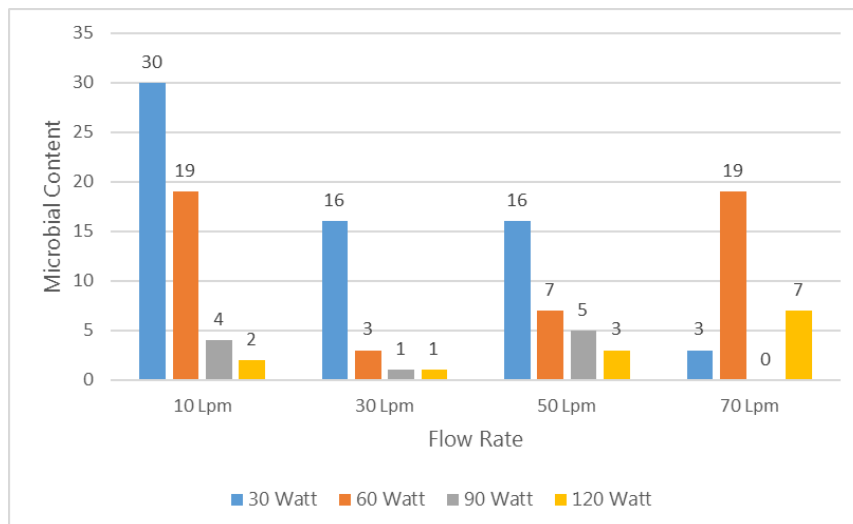
Figure 4: TPC Result Using Filtration of Carbon Active
