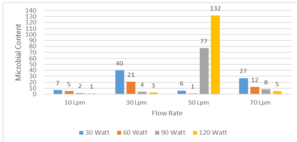
Figure 3: TPC Result Using Filtration of Crumb Rubber
