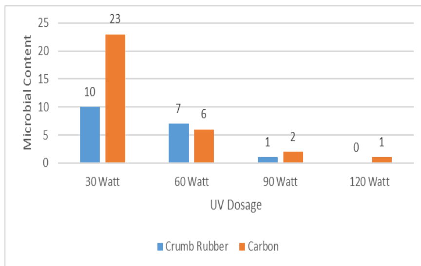
Figure 6: Comparison of Crumb Rubber and Carbon on 10 6 Dilution with flow Rate 10 Lpm
