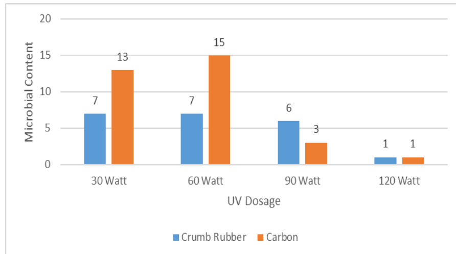
Figure 5: Comparison of Crumb Rubber and Carbon on 10 5 Dilution with flow Rate 10 Lpm
